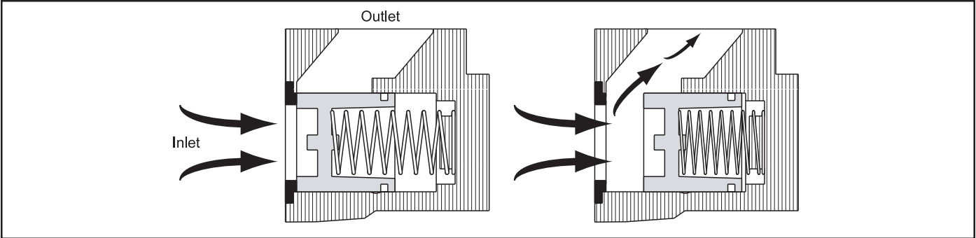
K-7 Valve Operation
